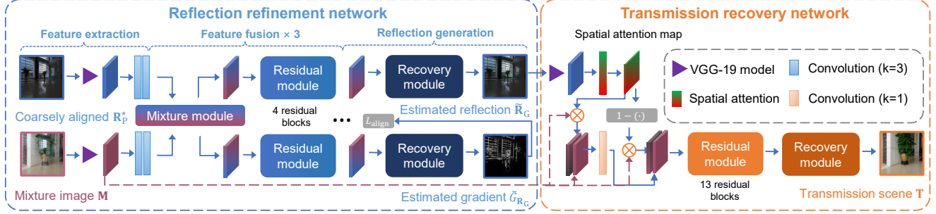
Figure 4. Illustration of detailed architectures of the reflection refinement network and the transmission recovery network. The reflection refinement network takes the coarsely aligned \mathbf{R}_p^* and \mathbf{M} as inputs and outputs an aligned reflection scene \tilde{\mathbf{R}}_G . The transmission recovery network estimates the transmission scene \mathbf{T} by taking \mathbf{M} and \tilde{\mathbf{R}}_G as inputs.
