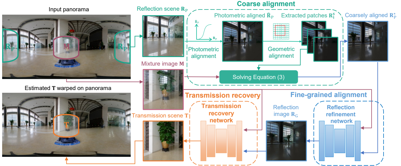
Figure 3. Given a panoramic image containing glass reflections with the mixture image M according to user-provided RoI, the panoramic reflection scene R_P is automatically cropped. Our method settles the geometric and photometric misalignment between the panoramic reflection scene and the glass-reflected reflection image with a coarse-to-fine strategy. For the coarse alignment, R_P is roughly aligned to the glass-reflected reflection image R_G via a pre-processing procedure with the help of M . Then a reflection refinement network for the fine-grained alignment takes the coarsely aligned R_P^c and M as inputs, outputting an aligned reflection image R_G . The transmission recovery network estimates the transmission scene T from M with the guidance of R_G and the estimated T is finally warped back to the panoramic image.
